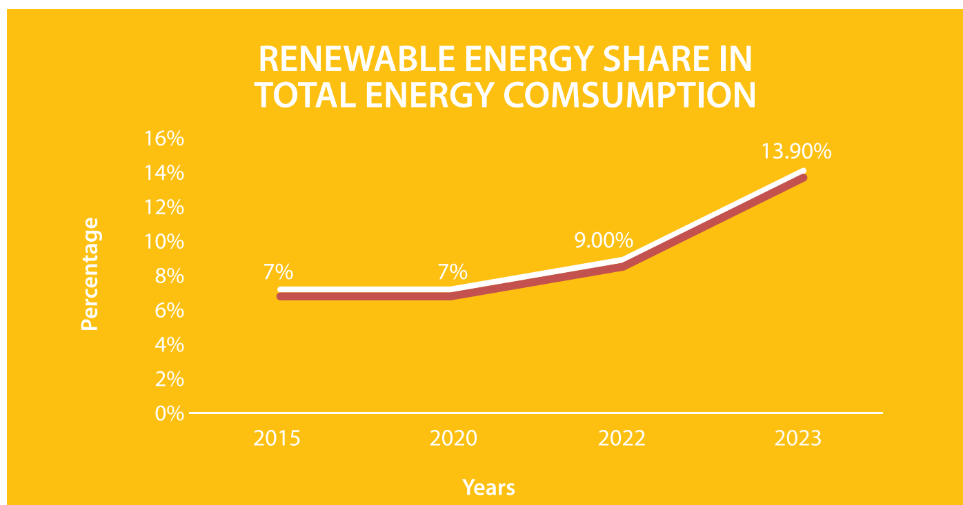
Figure 13: Renewable energy share in the total final energy consumption
